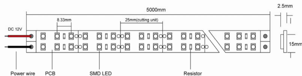
3528 LED STRIP 600LEDs/5m 48W DC12V/24V IP68 waterproof
