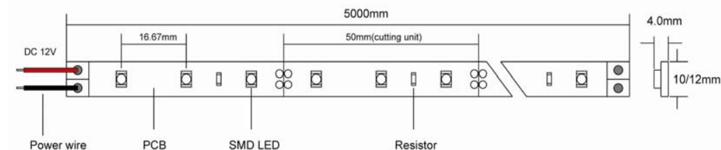
3528 LED STRIP 300LEDs/5m 24W DC12V/24V IP68 waterproof ( covered with tube )
