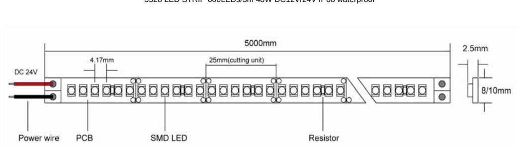
3528 LED STRIP 600 LEDs/5m 18W DC12V/24V IP68 waterproof
