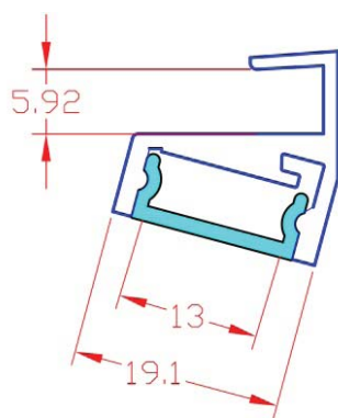
LED Profile G001 For 6mm glass shelf
