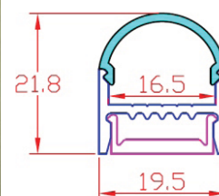
LED Profile D001 Designed for dual line LED strips
