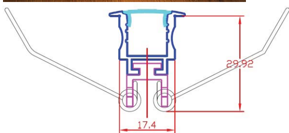
LED Profile A2520 Recessed Profile with Spring Clips
