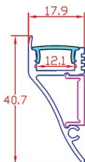
LED Profile W001 Designed for wall decoration
