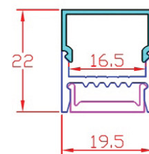
LED Profile D002 Designed for dual line LED strips
