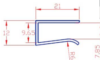
LED Profile G003 8mm glass edge lighting profile
