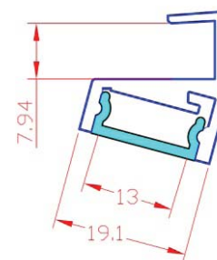
LED Profile G002 For 8mm glass shelf
