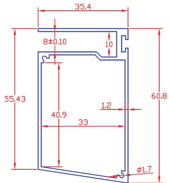
LED Profile G004 Glass Shelf Profile with LED Driver
