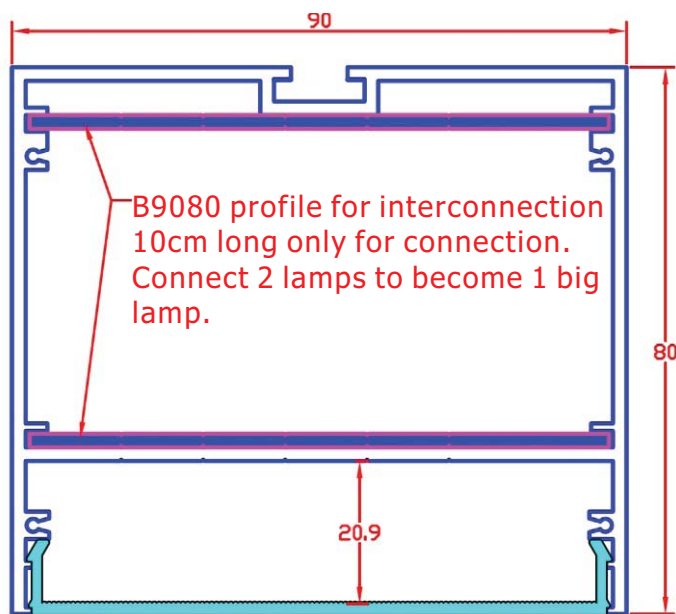
LED PROFILE A9080 Pendant Profile with LED Driver inside
